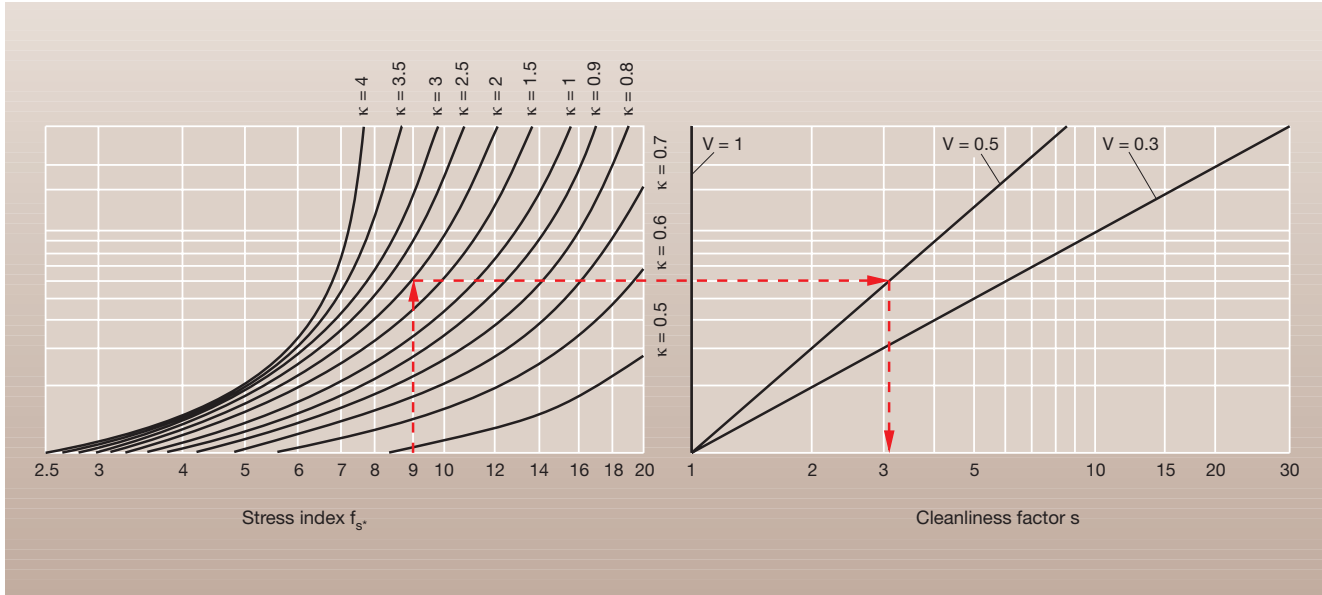
22: Diagram for the determination of cleanliness factor s
